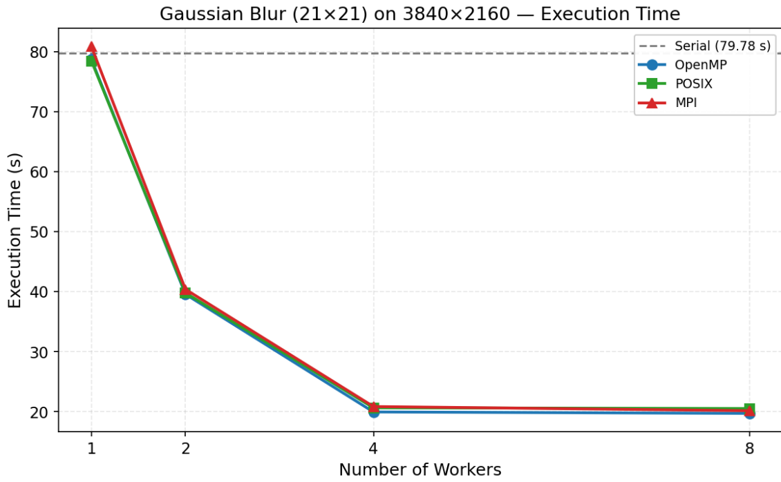
Figure 9: Execution time vs. worker count for Gaussian blur.
