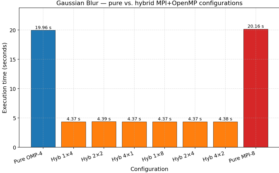
Figure 11: Hybrid vs. pure implementation execution times for the Gaussian blur. The hybrid configurations cluster around 4.5 s — roughly 4.5× faster than pure OpenMP/MPI at the same worker count.
